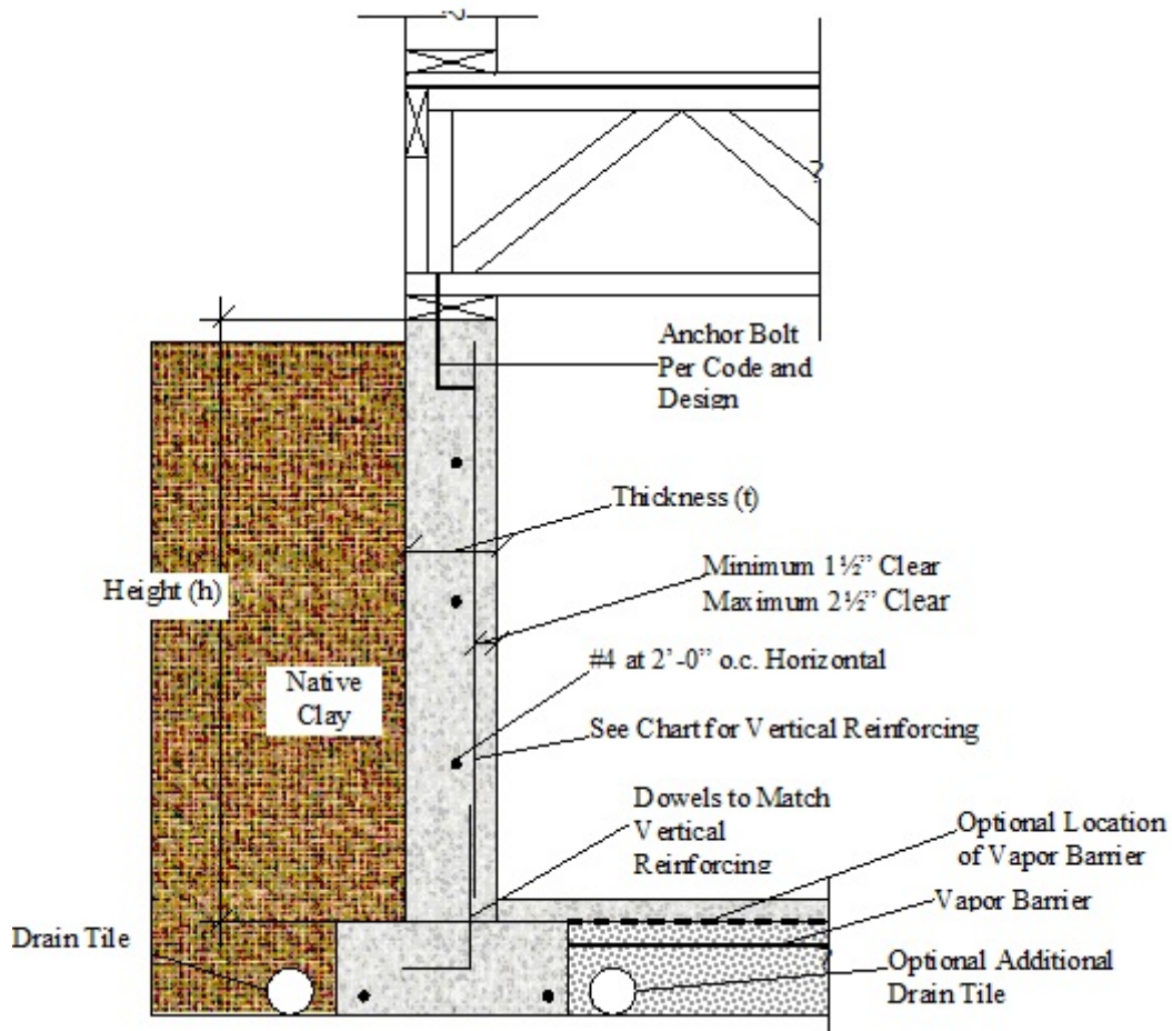
FIGURE R404.1.2 (2)
